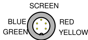
5 WAY CABLE PLUG (VIEW ON PINS SHOWING WIRE COLOURS)
